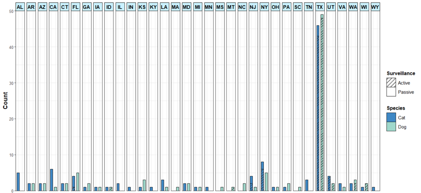
Supplementary Figure S1 —SARS-CoV-2 positive cats (n=109) and dogs (n=95) cases reported by state. Companion animals were identified through either passive or active surveillance.
