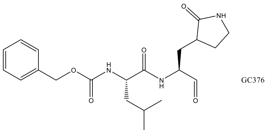
Figure S13 Mass of positive control GC376.
