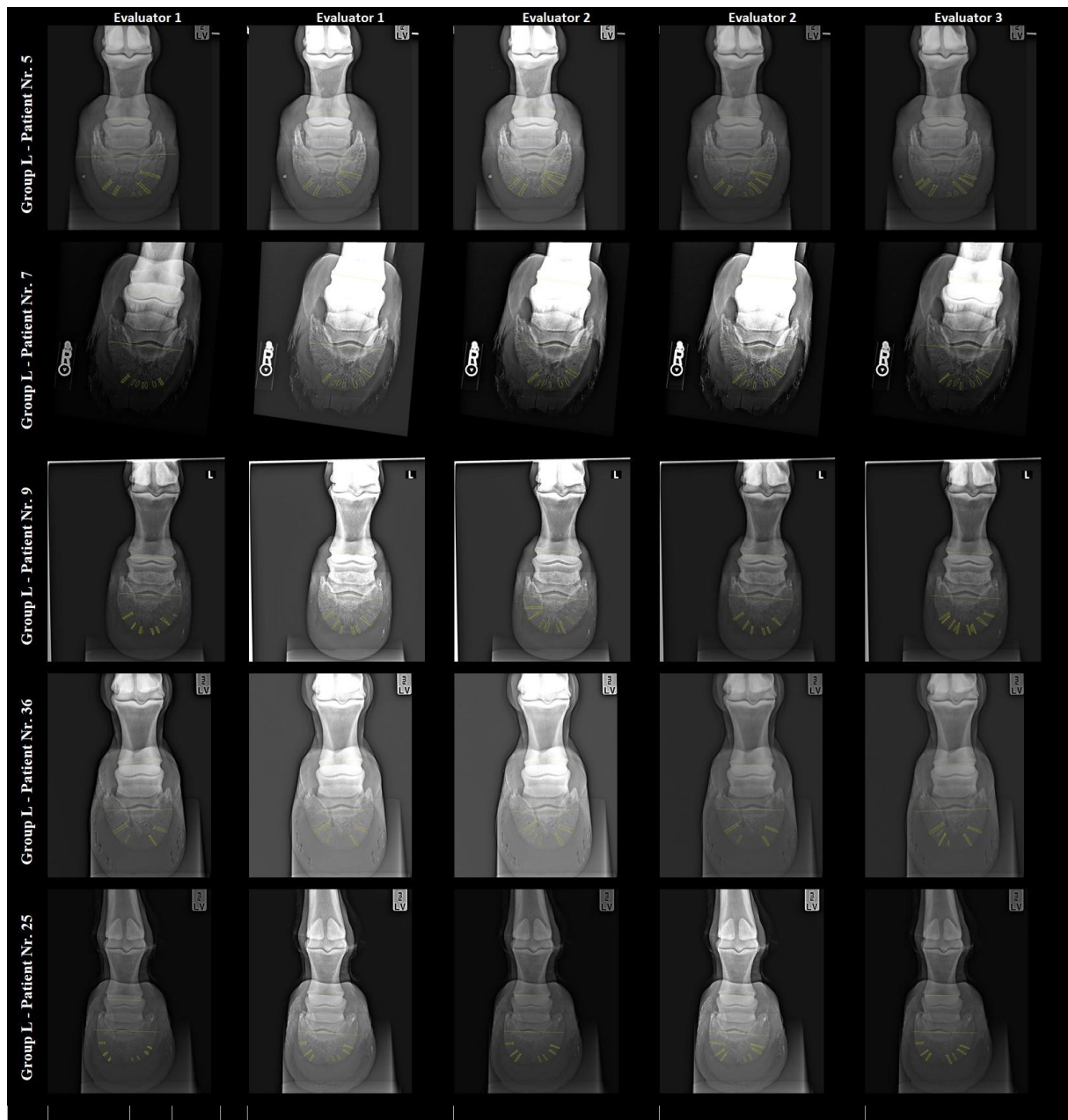
Supplementary Figure S3 – The first, third, fourth and fifth row show Oxspring (0°; dorsoproximal–palmarodistal) and the second row show High Coronar (65°; dorsoproximal–palmarodistal) radiographic views of 5 forefeet of 5 horses of Group L (with laminitis) to illustrate the first measurements to test the repeatability and reliability of the software. Three human evaluators measured the same 5 radiographs, and evaluator 1 and 2 remeasured the same radiographs a second time.
