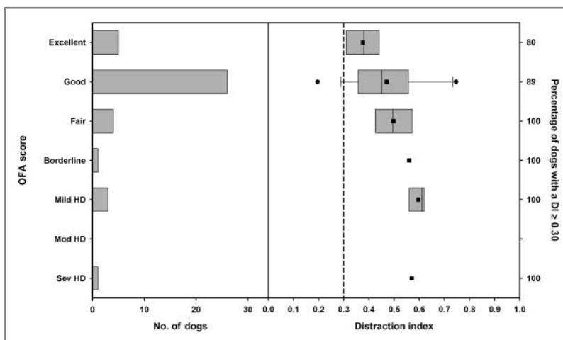
Figure 3—Distribution of OFA scores (left) and associated box-and-whisker plots of DIs (right) for 40 Labrador Retrievers \geq 2 years of age that underwent routine hip joint screening at a veterinary teaching hospital from June 1987 through July 2008. See Figure 1 for key.
