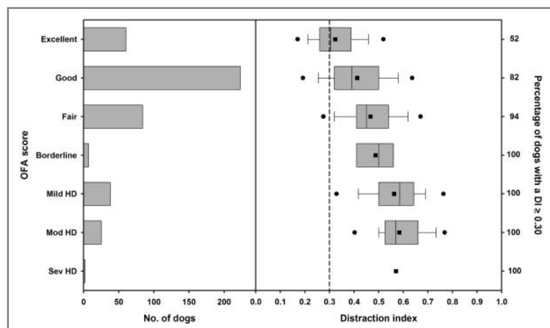
Figure 1—Distribution of OFA scores (left) and associated box-and-whisker plots of DIs (right) for 439 dogs \geq 2 years of age of various breeds that underwent routine hip joint screening at a veterinary teaching hospital from June 1987 through July 2008. In the box plots, the vertical line within each box represents the median, the square in the center represents the mean, the vertical edges of each box represent the 25th (left) and 75th (right) percentiles, and the whiskers represent the 10th (left) and 90th (right) percentiles. Circles represent the 5th and 95th percentiles. The vertical line at a DI of 0.3 indicates the cutoff used to designate osteoarthritis-nonsusceptible ( < 0.30 ) and osteoarthritis-susceptible ( \geq 0.30 ) dogs. HD = Hip dysplasia. Mod = Moderate. Sev = Severe.
