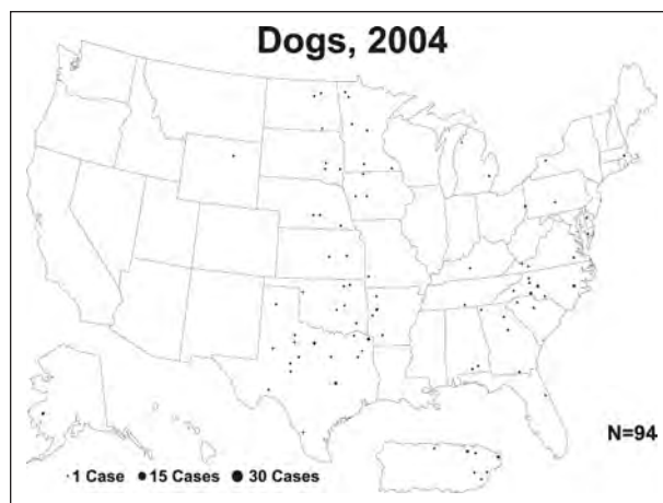
Figure 12—Reported cases of rabies in dogs, by county and municipio (Puerto Rico), 2004.
