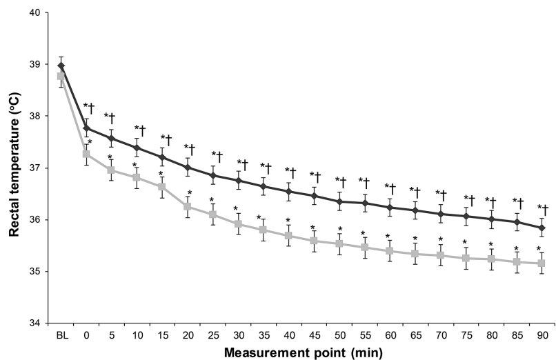
Figure 1 —Mean rectal temperatures recorded at hospital intake (baseline [BL]) and prior to (0 minutes) and every 5 minutes after anesthetic induction for 23 adult dogs undergoing routine ovariohysterectomy. All dogs were premedicated with buprenorphine and acepromazine. Anesthesia was induced with midazolam or diazepam (0.25 mg/kg, IV) plus ketamine hydrochloride (5 mg/kg, IV; diamonds [ n = 11 ]) or propofol (4 mg/kg, IV; squares [12]). Error bars represent SD. *Value differs significantly ( P \leq 0.05 ) from respective BL value. †Value differs significantly ( P \leq 0.05 ) between groups at the indicated measurement point.
